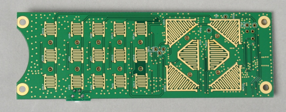
Light Weight Tactical Handset, PCB Top View SA-20935
