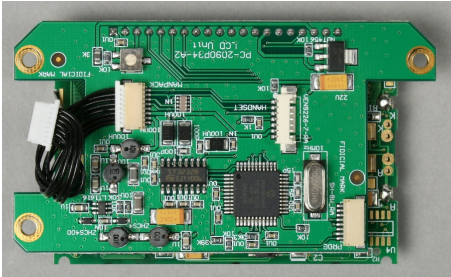
PRC-2090 LCD Unit Internal Boards, Assembled LCD Unit PC Board, Top View Shown PC-2090P34
