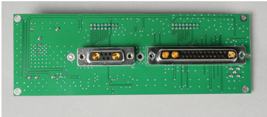
Cradle Interface PCB, Bottom View SA-20908
